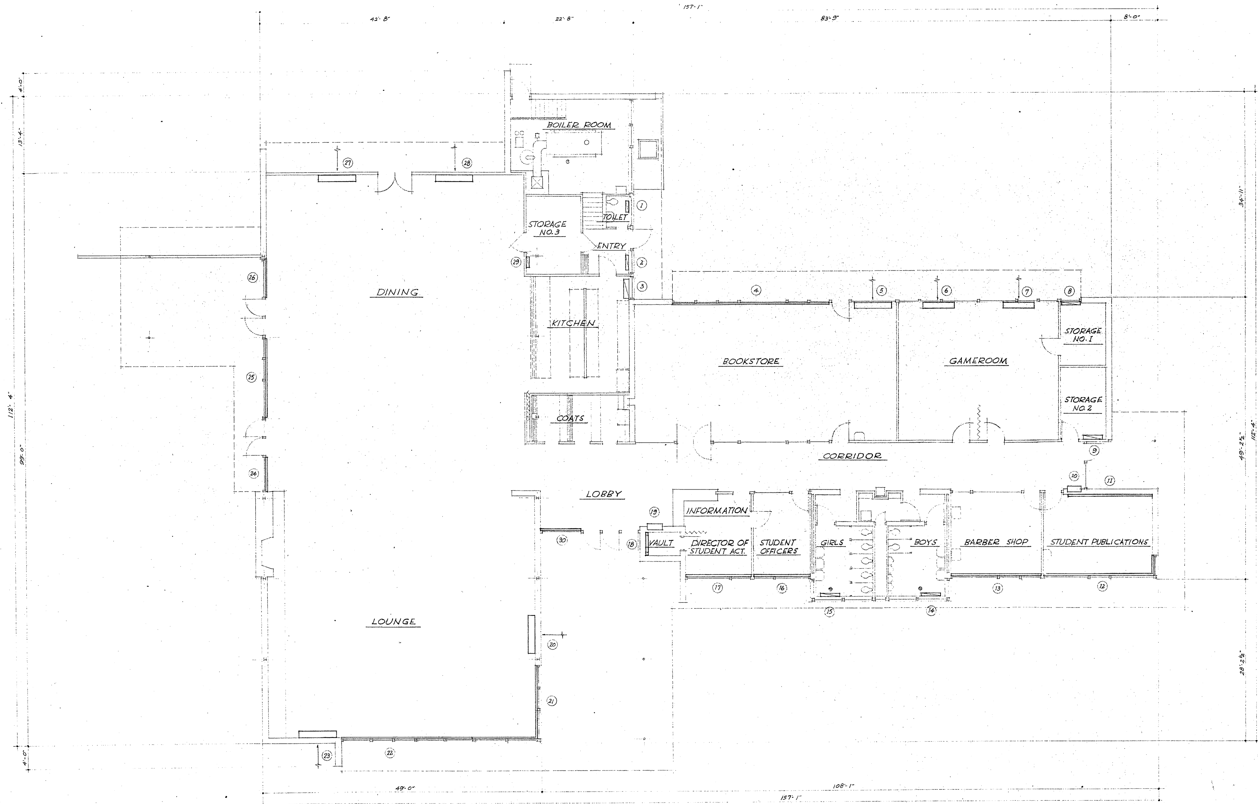
HEATING FIRST FLOOR PLAN 8"=1'-0"
