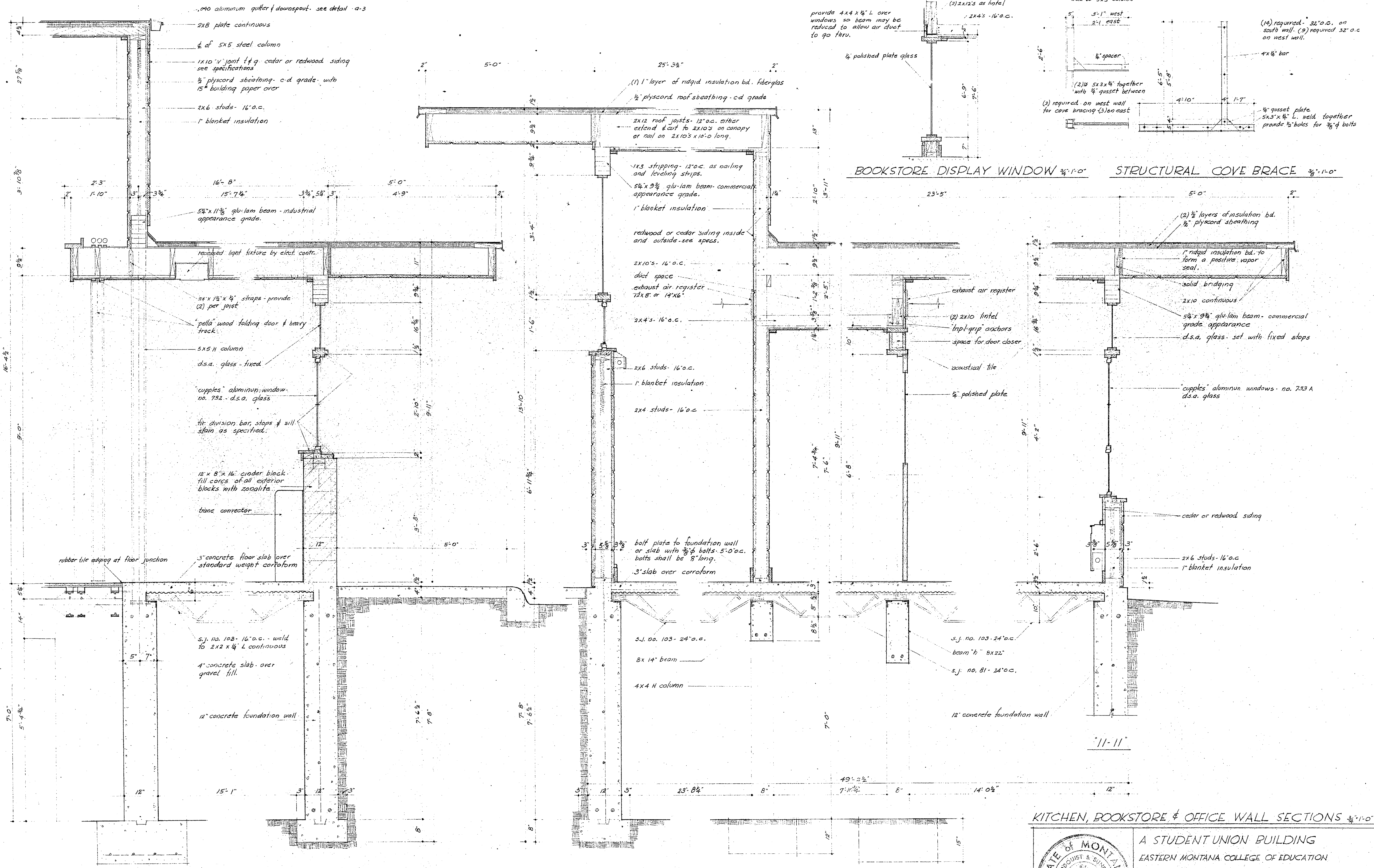
WALL SECTIONS 6-6
