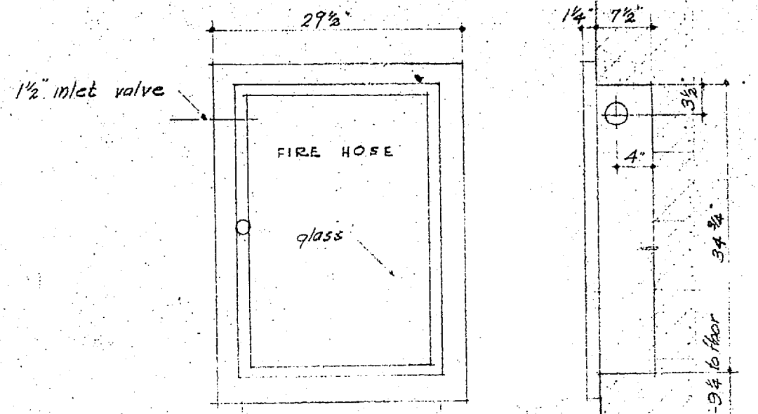
FIRE HOSE CABINET 3/8" = 1'-0" one required by plumbing & heating contr.
