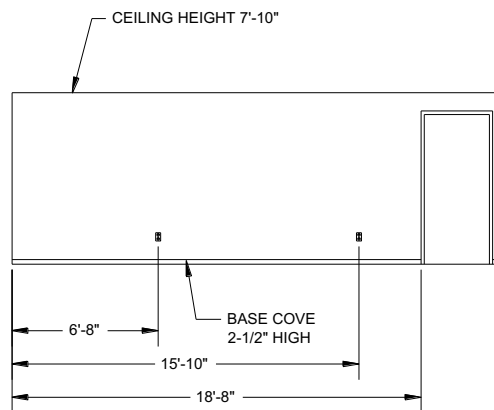
NORTH ELEVATION
